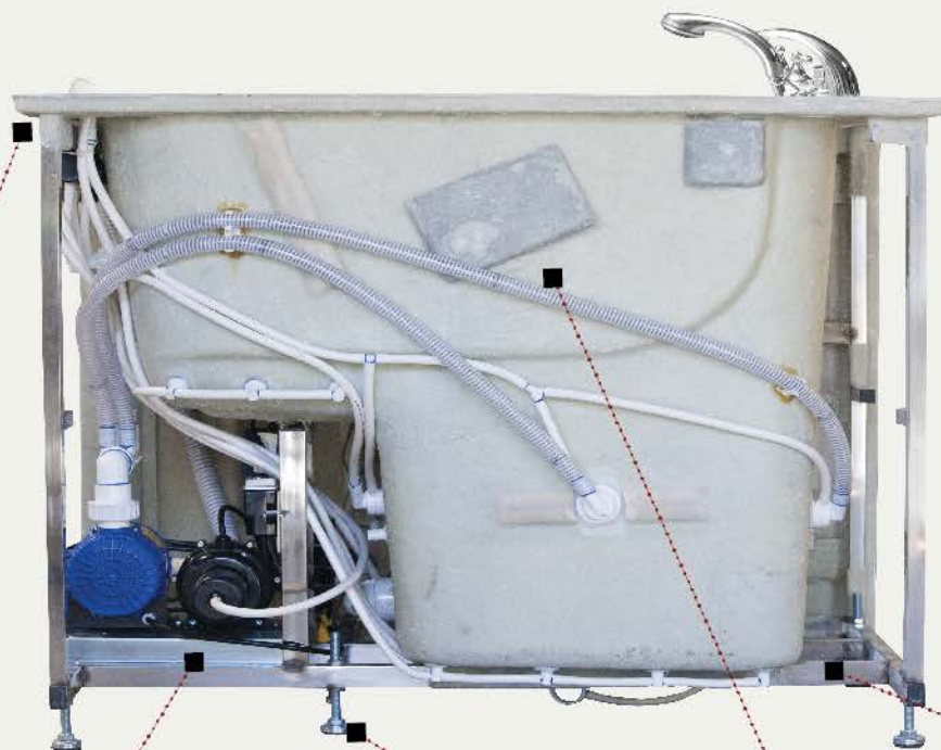
Motor Placement
